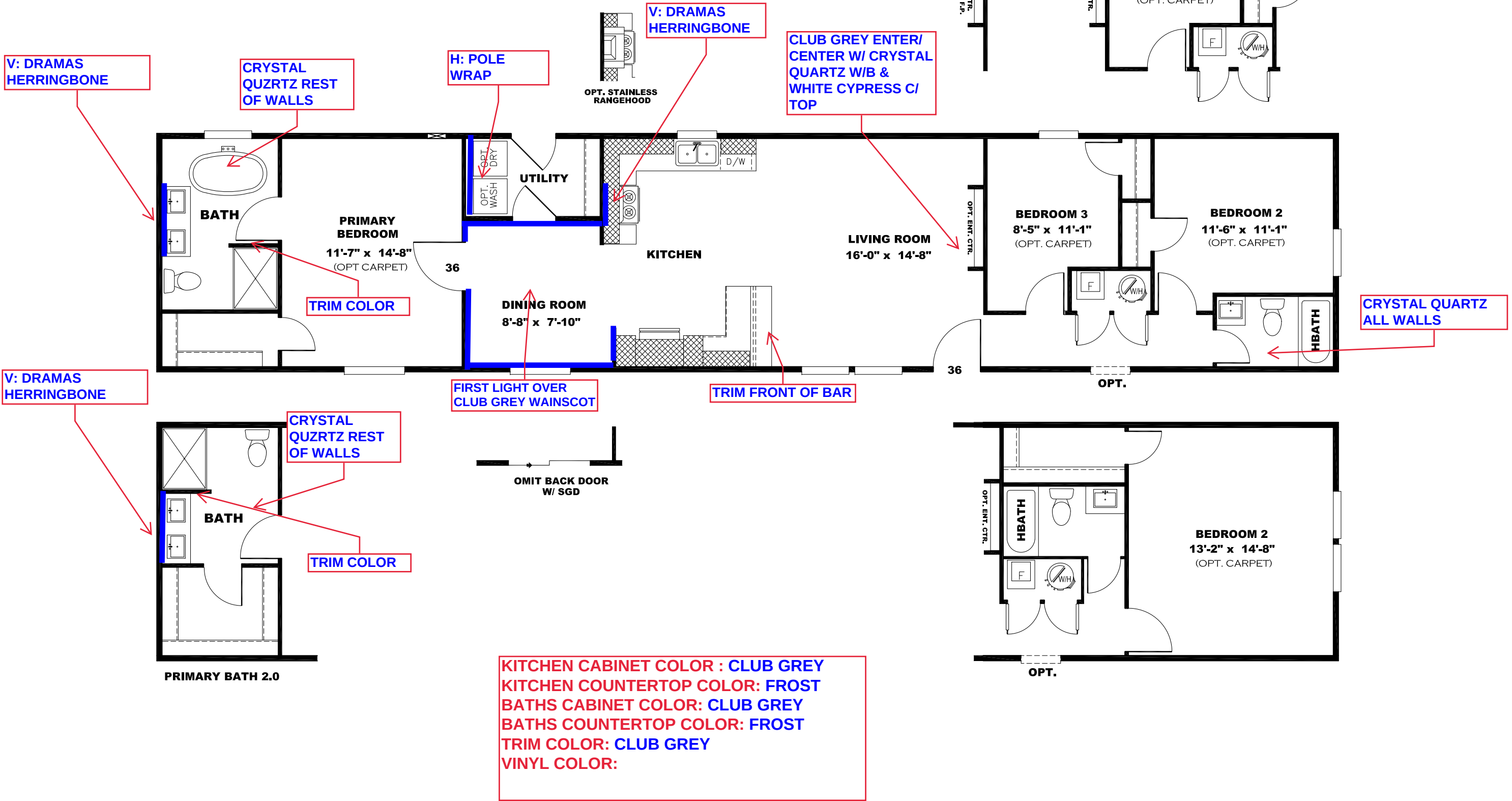
DRAWING# LFS-22S096 MODEL# LFS16763Q 16' X 76' LIFESTYLE
